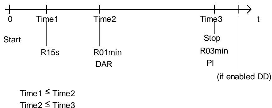
Fig. 19. Timer relations
